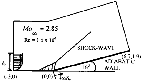
Fig. 9 Schematic diagram of the 16° ramp flow at Ma_\infty=2.85
