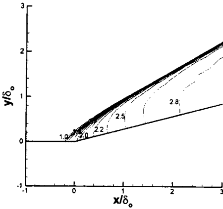
Fig. 10 Dimensionless pressure contours over the 16° ramp
