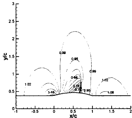
Fig. 4 Dimensionless pressure contours over the axisymmetric bump
