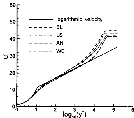
Fig. 2 Logarithmic velocity profiles for the compressible flat plate flow at Ma_\infty=2.83
