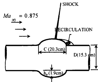
Fig. 3 Schematic diagram of an axisymmetric bump flow at Ma_\infty=0.875
